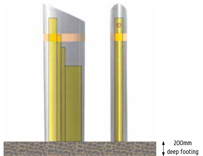
Foundation only 200mm deep x 900mm wide x 1200mm long Tested and passed as a single removable bollard
